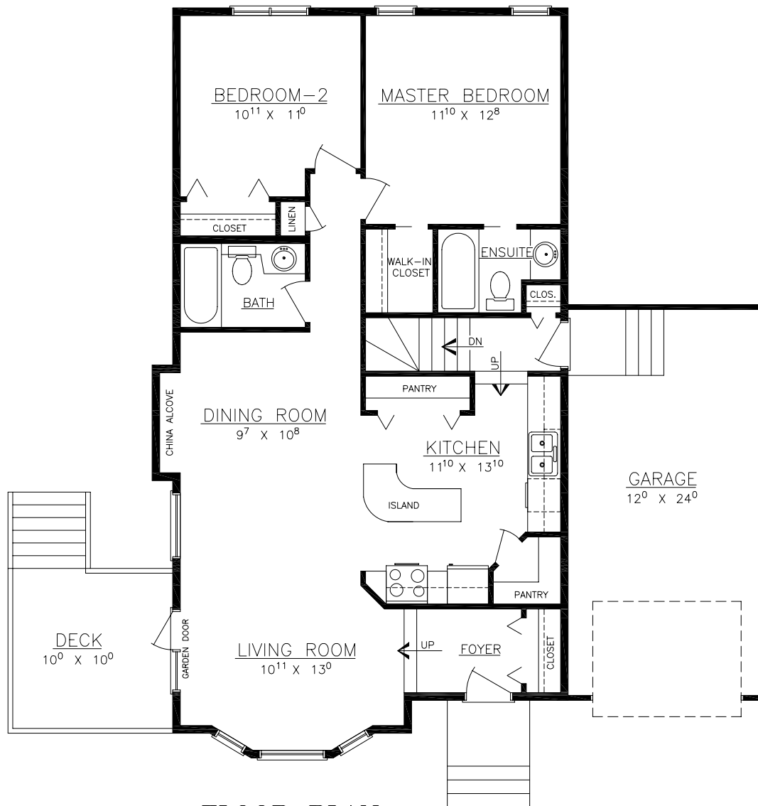
FLOOR PLAN
